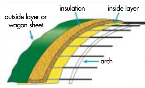
Exploded view of the cover and insulation.
